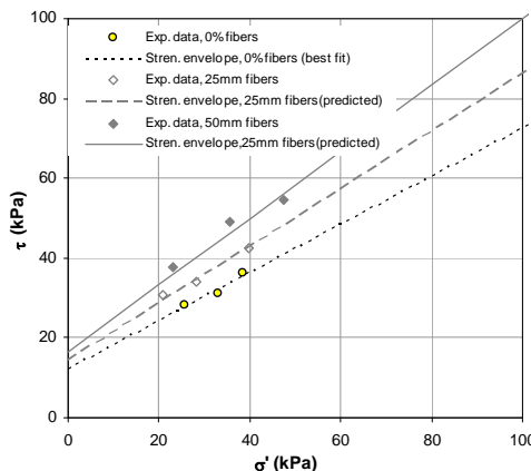
Figure 23 Comparison between predicted and experimental shear strength results for specimens reinforced at \chi_w =0.4\% , with 25 mm-long and 50 mm-long fibers (2610 denier), Soil 2
