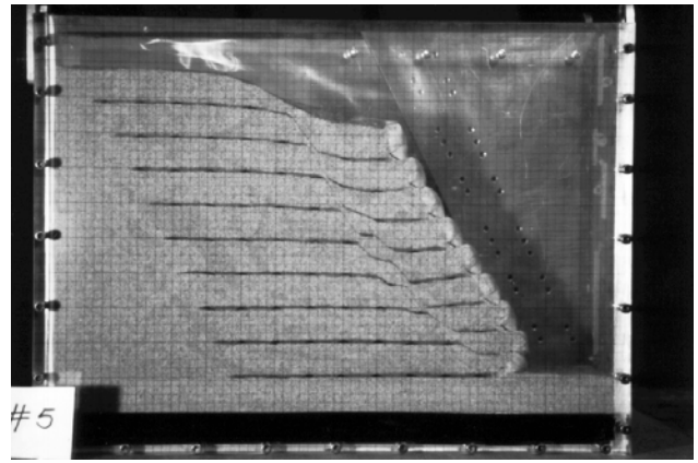
Figure 6. Failed geotextile-reinforced slope model.
