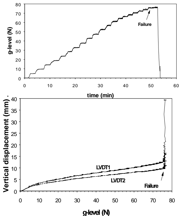
Figure 4. G-level (N) versus time during centrifuge testing.
