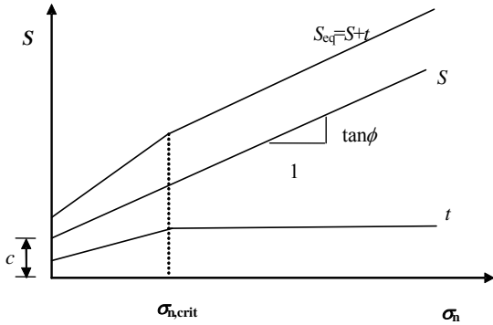
Figure 11 Representation of the equivalent shear strength according to the discrete approach
