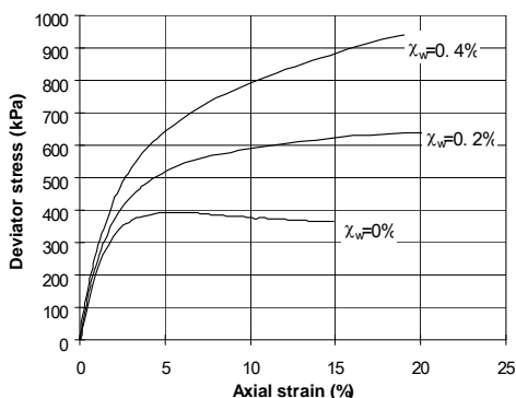
Figure 13 Stress-strain behavior of specimens prepared using \chi_w = 0, 0.2 and 0.4\% with l_f = 25 mm fibers (360 denier), \sigma_3 = 140 kPa, Soil 1
