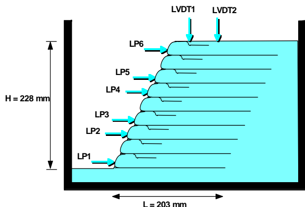
Figure 1. Typical centrifuge model.
