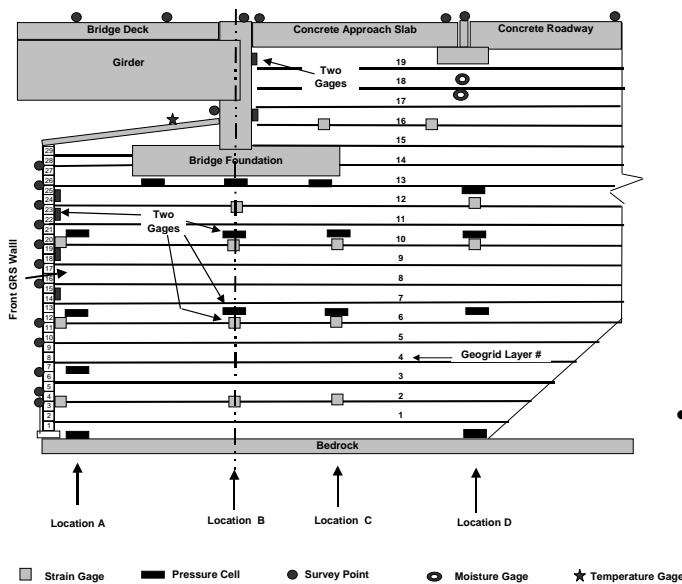
Figure 10. Instrumentation plan of Phase II structure.
