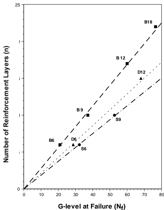
Figure 8. G -level at failure for the centrifuge models.
