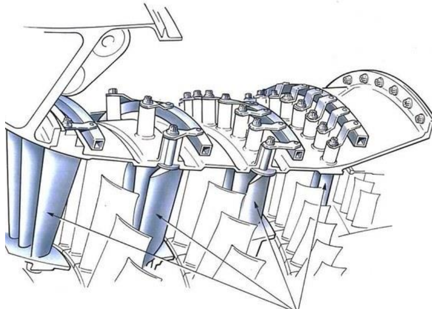
VARIABLE STATOR VANES
