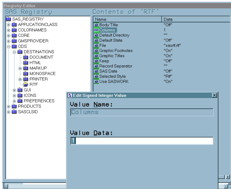
Display 10.8 Registry Editor Window
