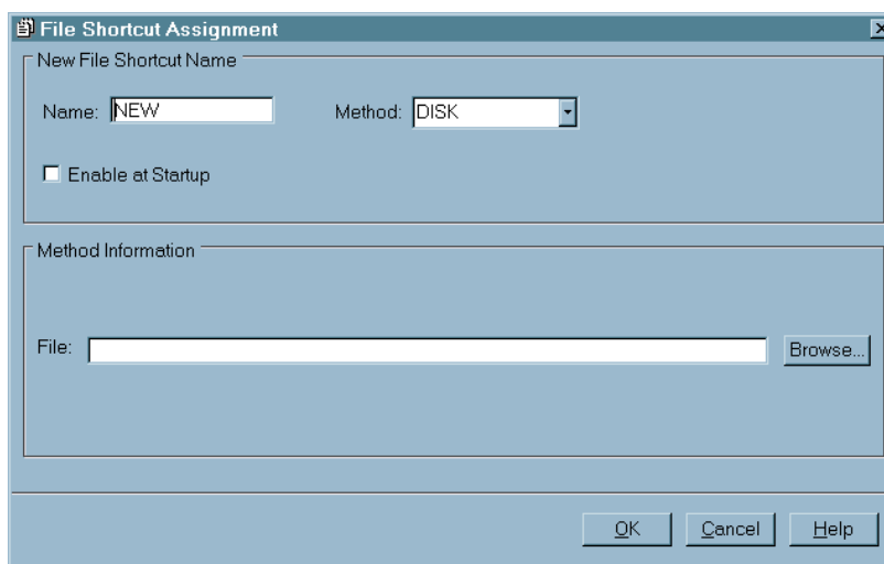
Display 18.12 File Shortcut Assignment Window
