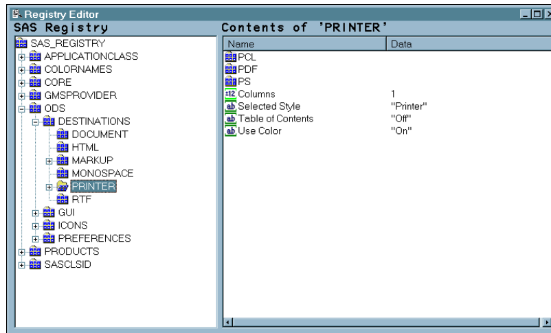
Display 10.6 SAS Registry of ODS Subkeys
