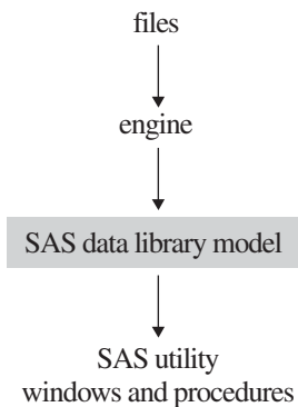
Figure 37.2 Relationship of Engines to SAS Data Libraries
