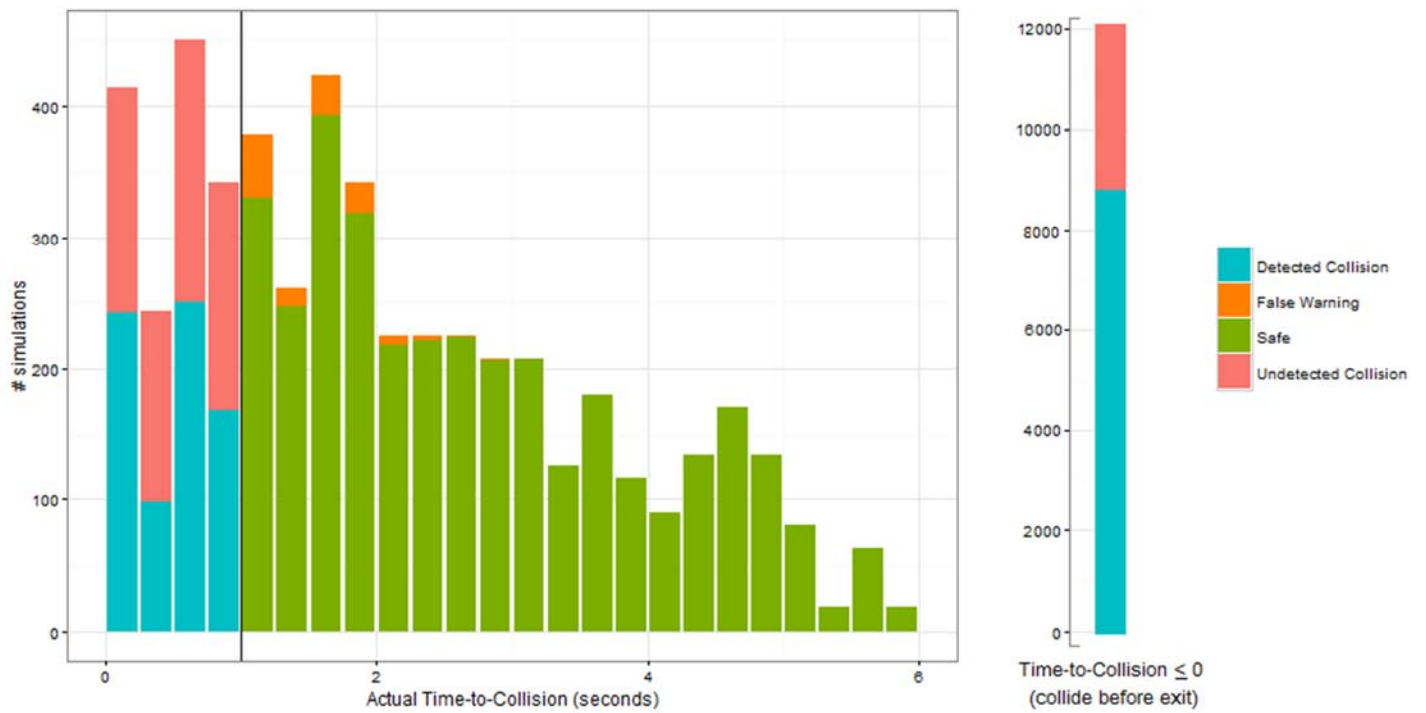
Figure 3: The actions of the overtaking assistant versus the actual time-to-collision between passing and oncoming vehicles
