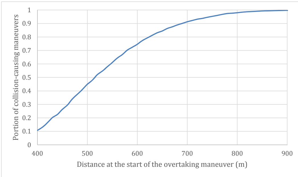
Figure 2: Cumulative distribution of collision maneuvers versus initial distance
