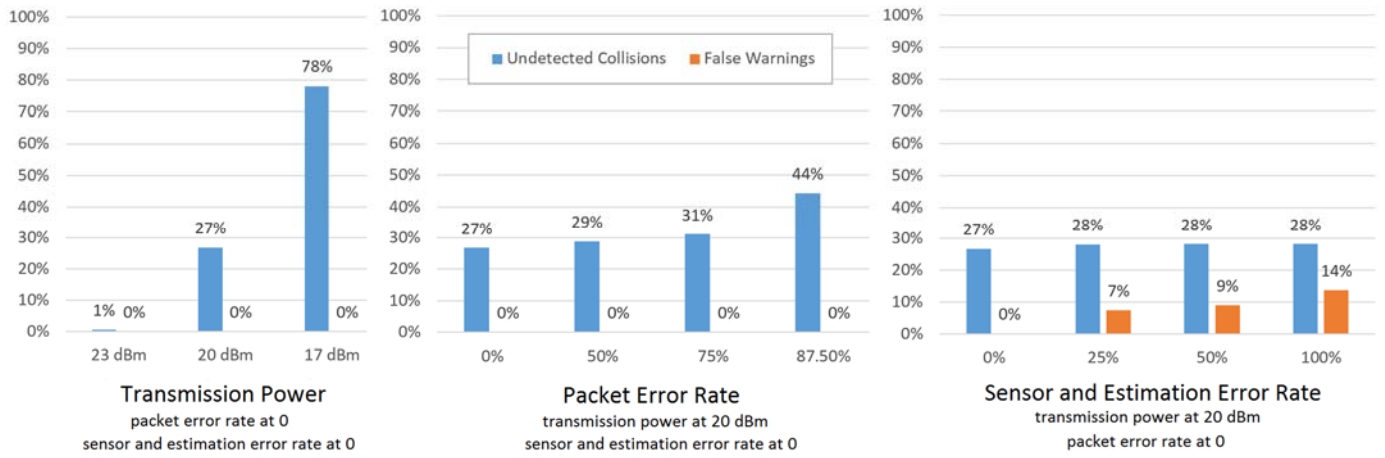
Figure 4: Overtaking assistant accuracy measures
